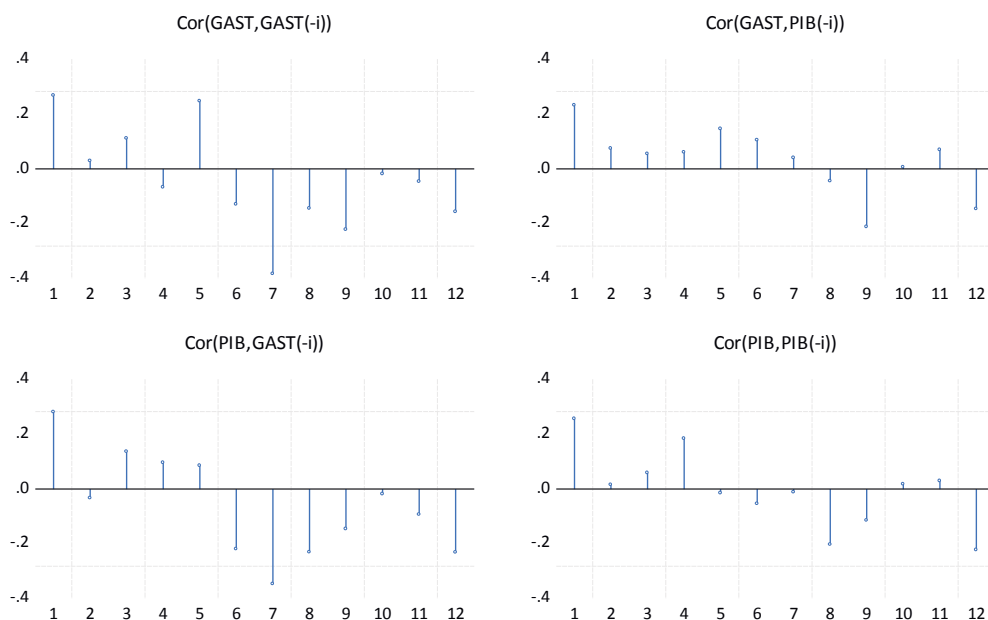
Figura 10. Test residual-correlograma
